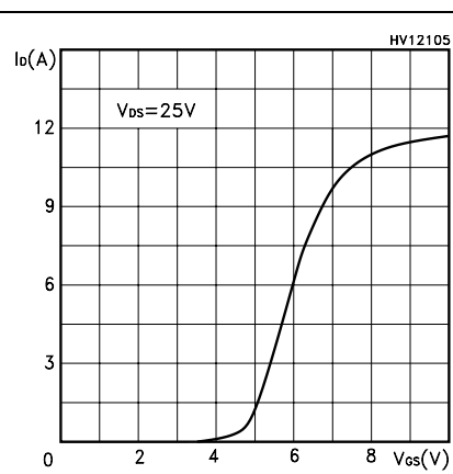
Figure 6. Transfer characteristics
