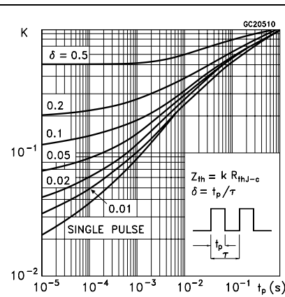
Figure 2. Thermal impedance for TO-220/ D 2 PAK/I 2 PAK
