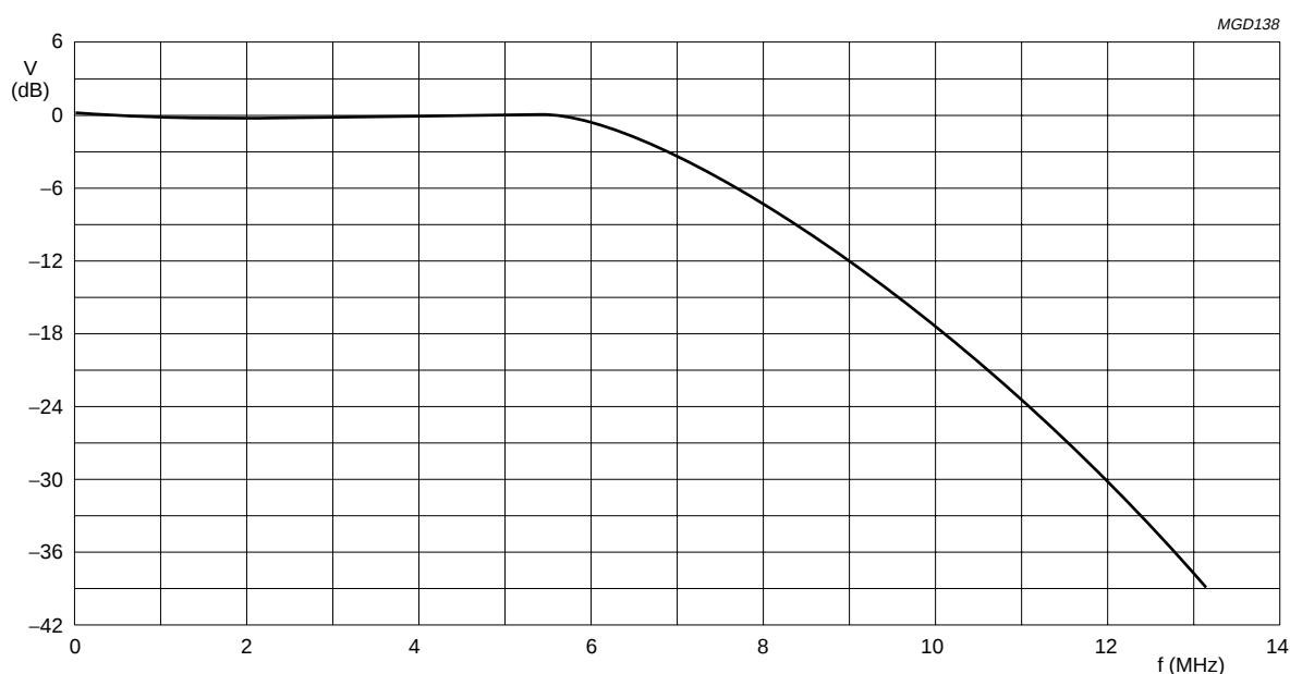
Fig.4 Anti-alias filter.
