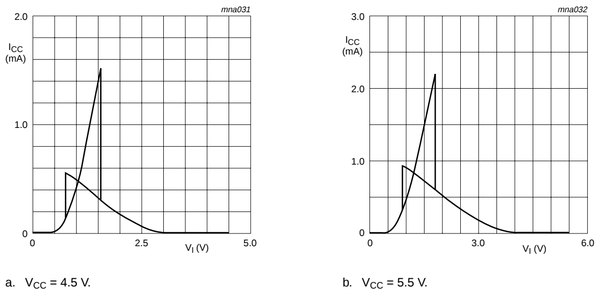
Fig 10. Typical 74HCT2G14 transfer characteristics
