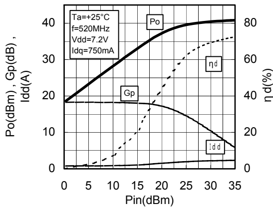
Pin-Po CHARACTERISTICS
