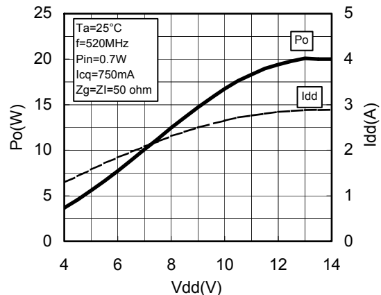
Vdd-Po CHARACTERISTICS
