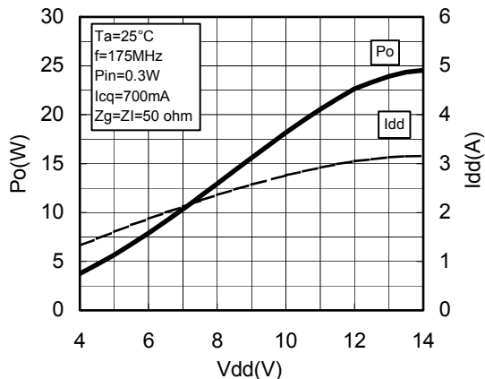
Vdd-Po CHARACTERISTICS
