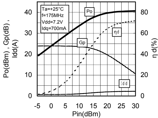
Pin-Po CHARACTERISTICS
