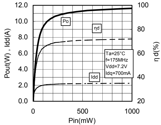
Pin-Po CHARACTERISTICS
