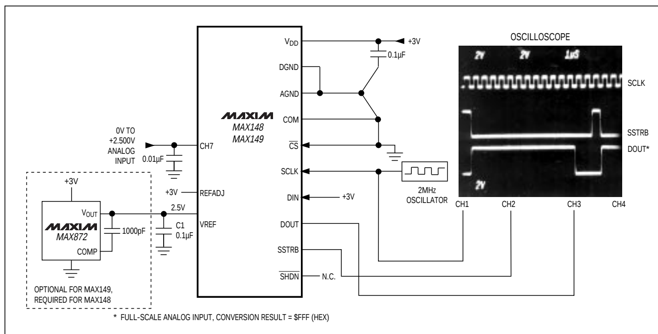
Figure 5. Quick-Look Circuit
