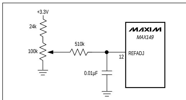
Figure 16. MAX149 Reference-Adjust Circuit
