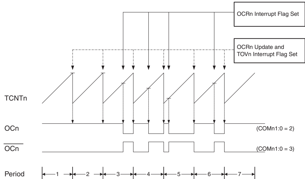
Figure 14-6. Fast PWM Mode, Timing Diagram
