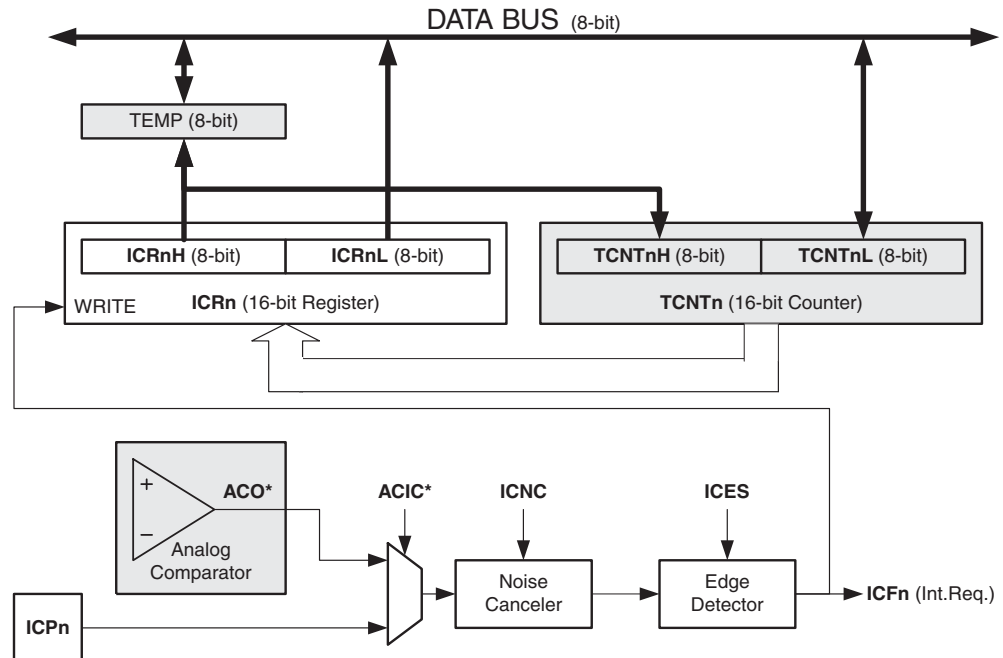
Figure 15-3. Input Capture Unit Block Diagram (1)
