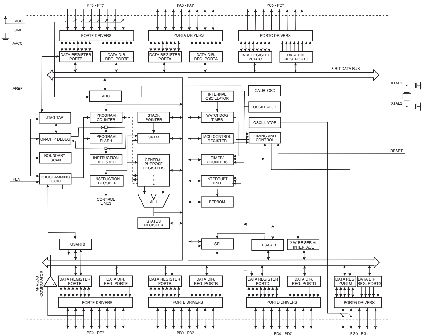
Figure 2-1. Block Diagram
