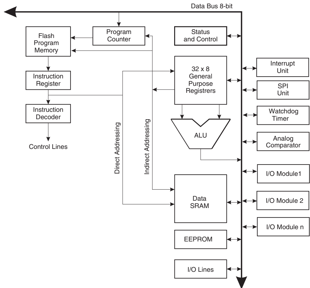
Figure 6-1. Block Diagram of the AVR MCU Architecture
