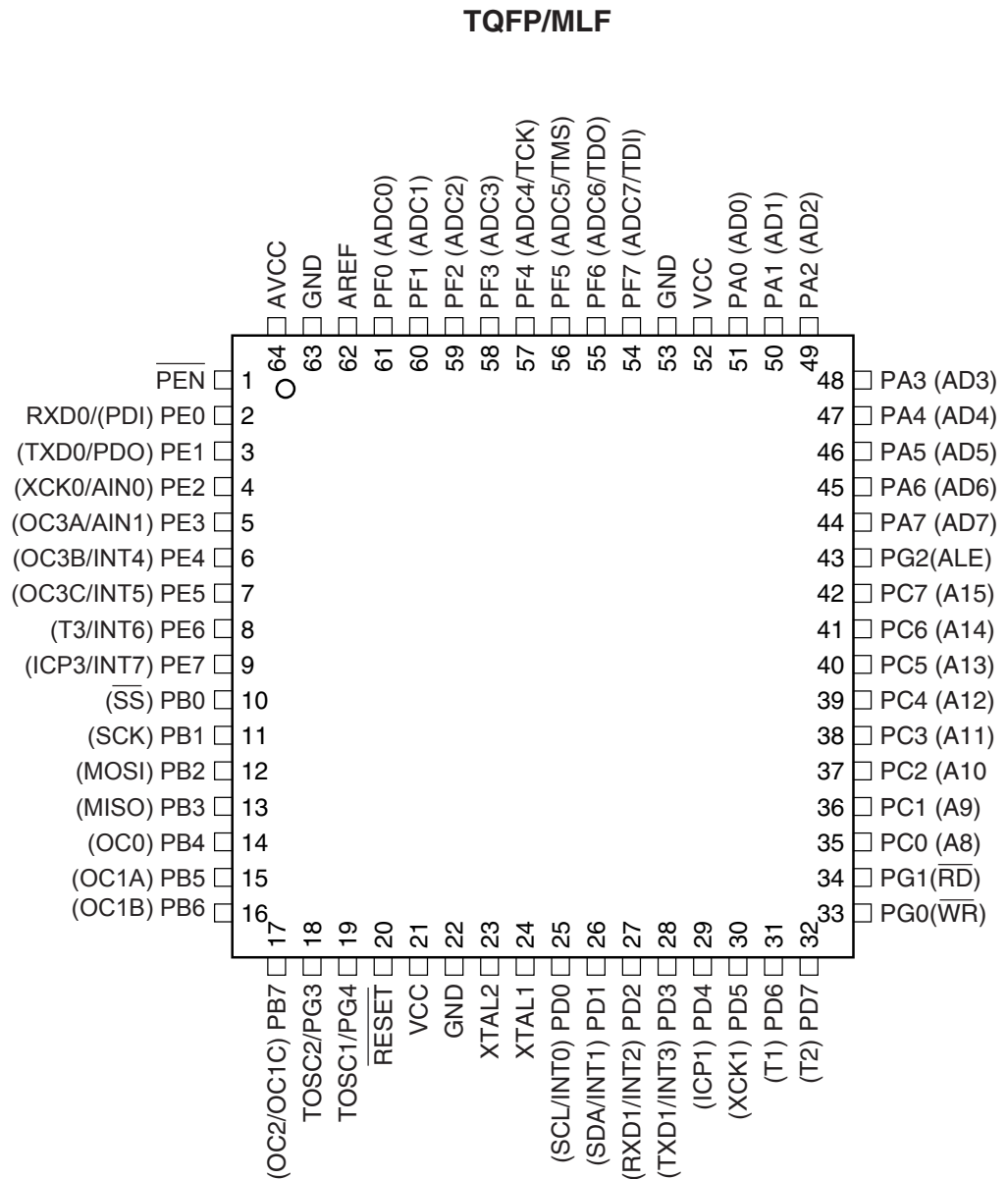
Figure 1-1. Pinout ATmega64A
