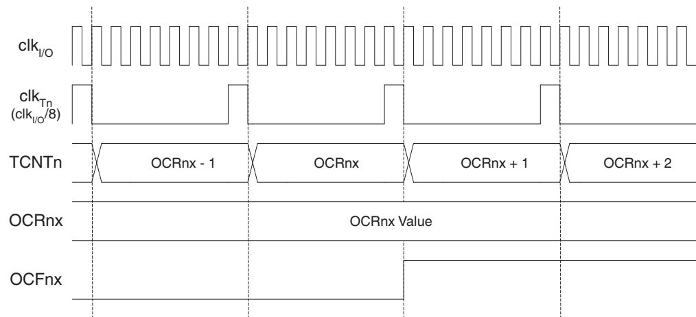
Figure 15-11. Timer/Counter Timing Diagram, Setting of OCFnx, with Prescaler ( f_{\text{clk\_I/O}}/8 )
