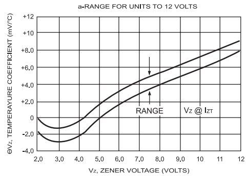
FIG.7- TEMPERATURE COEFFICIENTS
