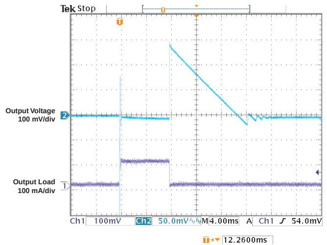
LOAD TRANSIENT RESPONSE VS TIME ( V_{\text{OUT}} = 5 \text{ V} , C_L = 10 \mu\text{F} )
