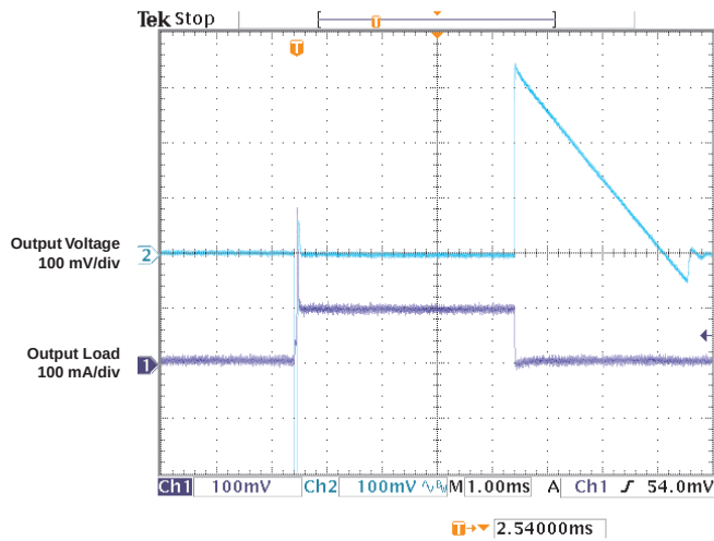
LOAD TRANSIENT RESPONSE VS TIME ( V_{\text{OUT}} = 5 \text{ V} , C_L = 1 \mu\text{F} )
