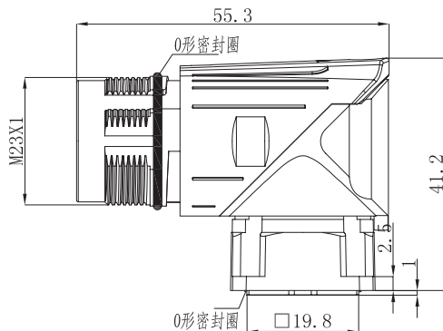
Heavy duty 90° angled socket
