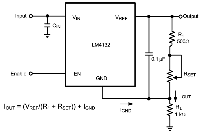
FIGURE 5. Programmable Current Source
