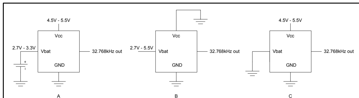
Figure 4. Power-Supply Connections
