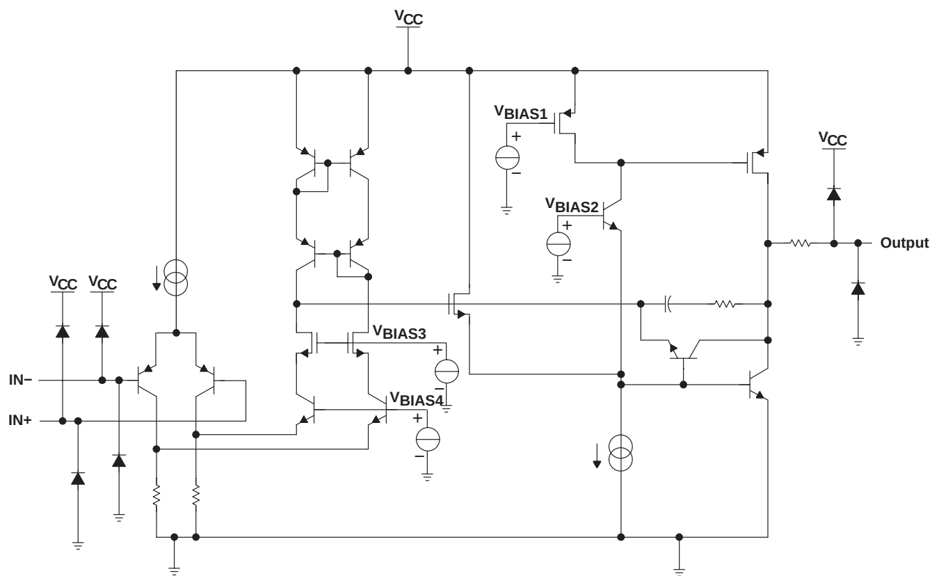
LMV324 simplified schematic
