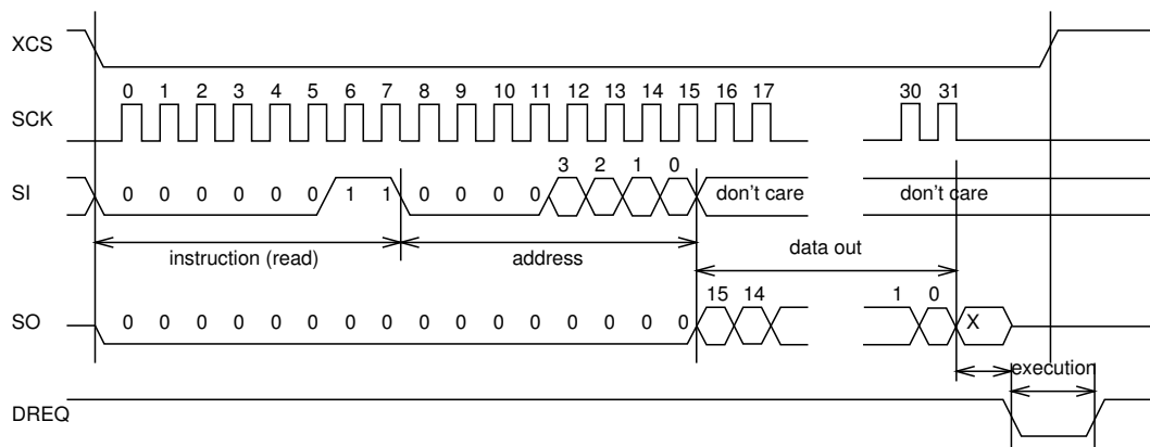
Figure 8: SCI Word Read
