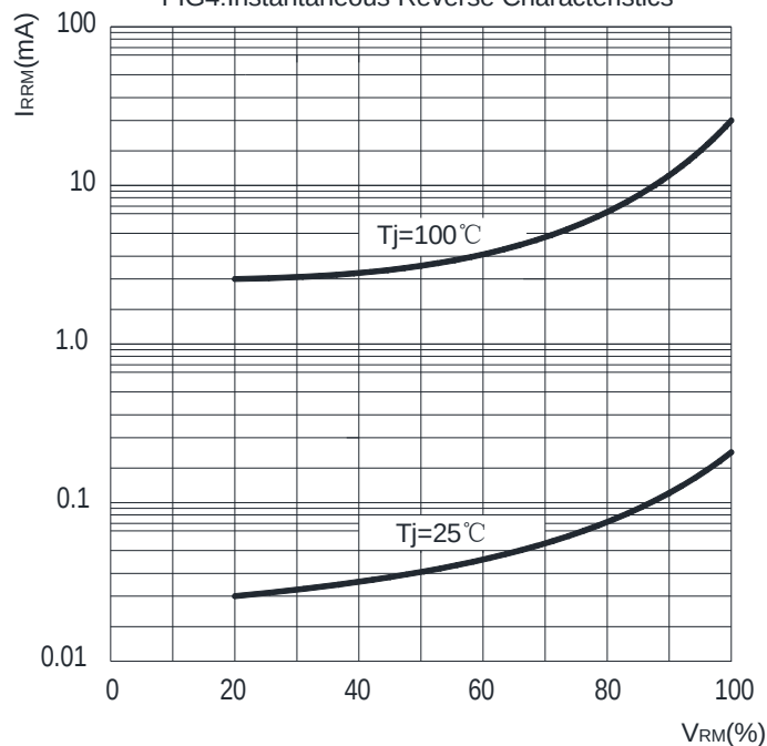
FIG4: Instantaneous Reverse Characteristics
