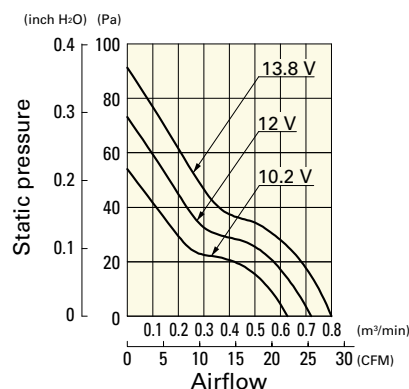
109R0612F401 With pulse sensor
