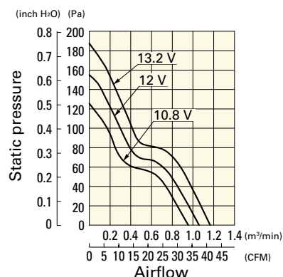
109R0612S401 With pulse sensor
