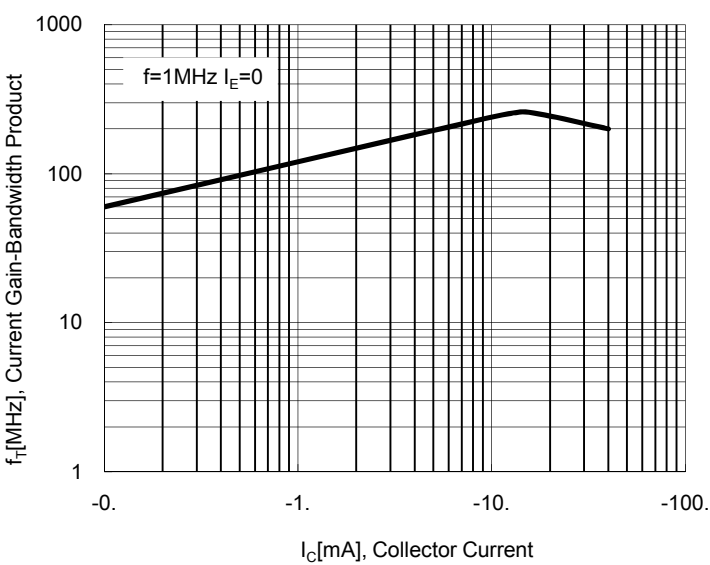
Fig. 6 Current Gain Bandwidth Product
