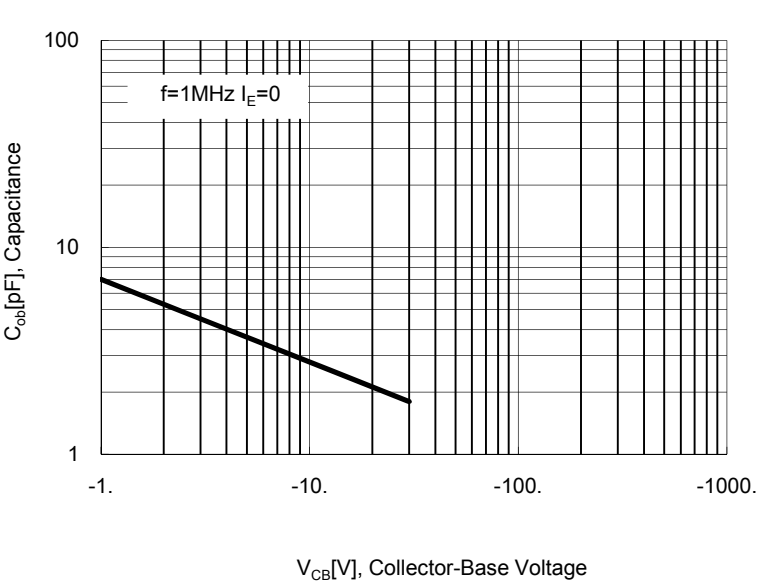
Fig.5 Collector Output Capacitance
