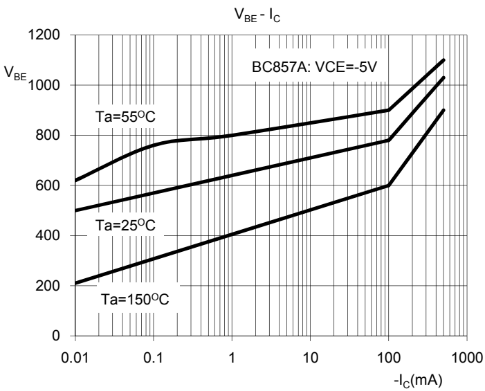
Fig. 8 Base-Emitter Voltage as a Function of Collector Current; Typical Values
