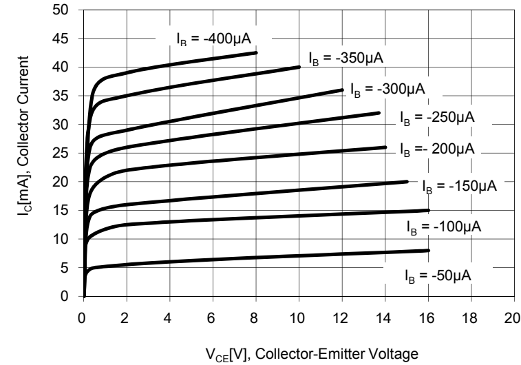
Fig. 1 Static Characteristic
