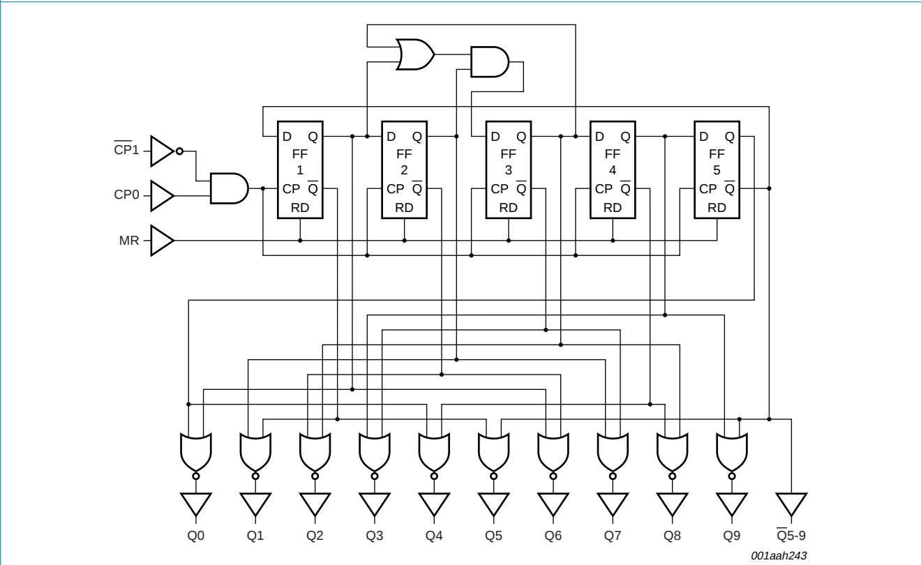
Fig 2. Logic diagram
