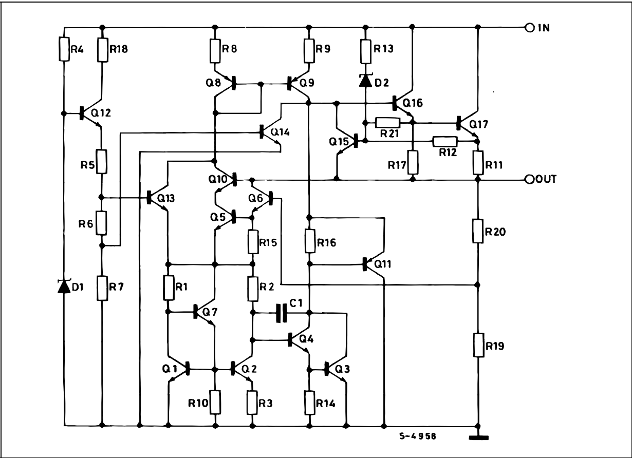
Figure 2. Schematic diagram
