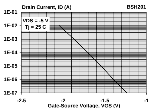
Fig. 11. Sub-threshold drain current. I_D = f(V_{GS}) ; conditions: T_J = 25 \text{ }^{\circ}\text{C}
