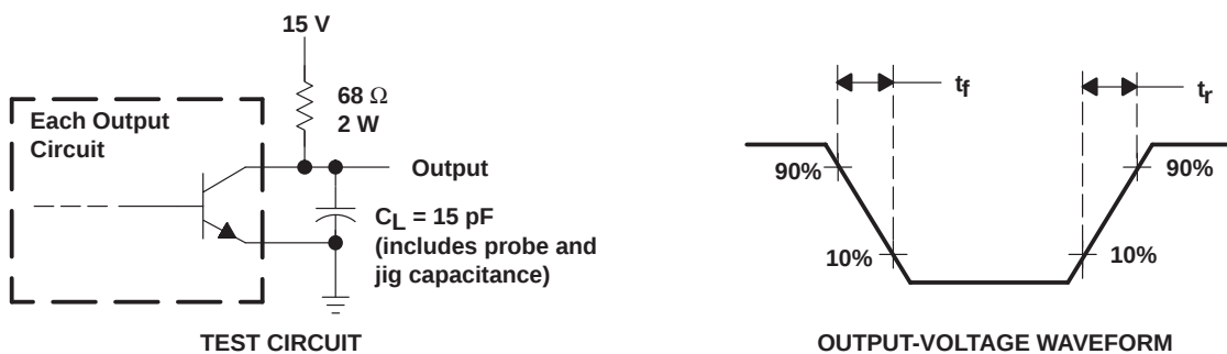
Figure 3. Common-Emitter Configuration
