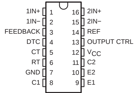
D, N, NS, OR PW PACKAGE (TOP VIEW)
