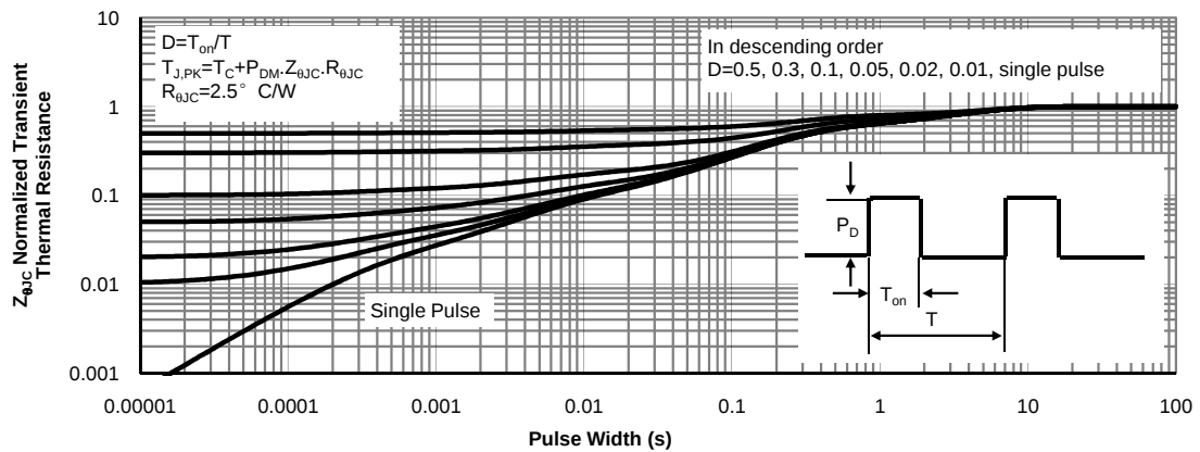
Figure 11: Normalized Maximum Transient Thermal Impedance for AOTF9N90 (Note F)
