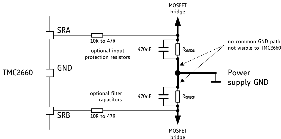
Figure 8.1 Sense resistor grounding and protection components
