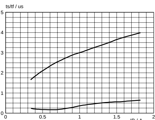
Fig. 10. Typical collector storage and fall time. t_s = f(I_B) ; \tau_f = f(I_B) ; I_C = 4.5 \text{ A} ; T_J = 85^\circ\text{C} ; f = 56 \text{ kHz}
