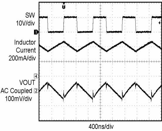
Switching Waveform
