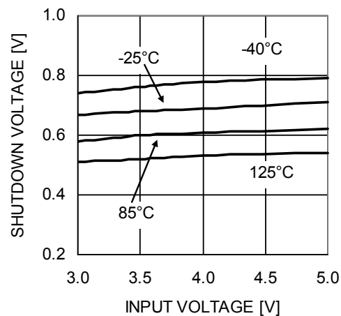
Shutdown Voltage
