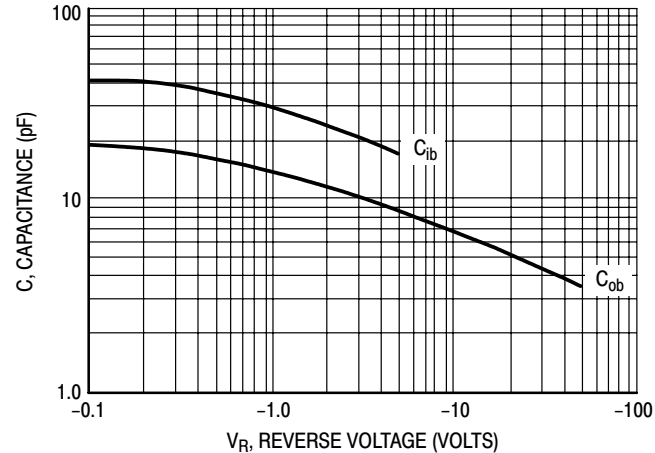
Figure 5. Capacitances
