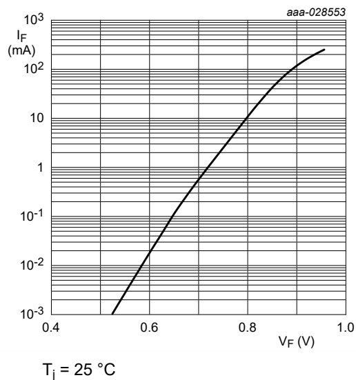
Fig. 5. Forward current as a function of forward voltage; typical values (BZT52H-B/C7V8)
