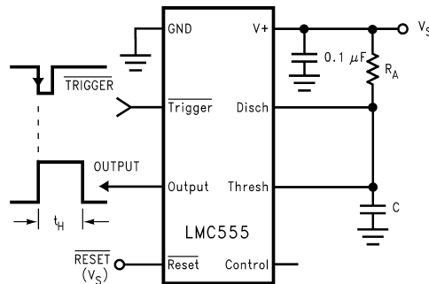
Figure 7-2. Monostable (One-Shot)
