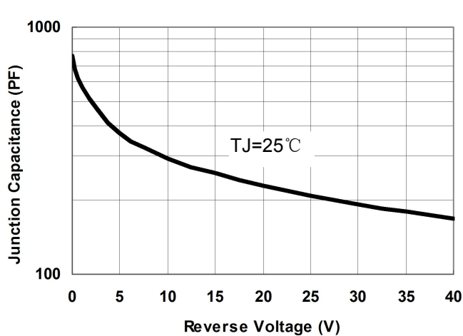
Fig.1-Typical Junction Capacitance
