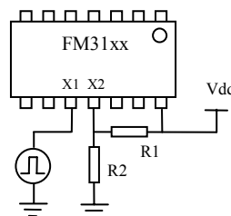
Figure 8. External Oscillator
