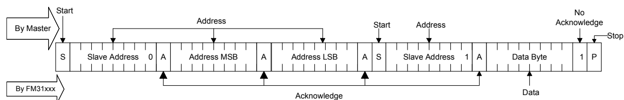
Figure 16. Selective (Random) Memory Read
