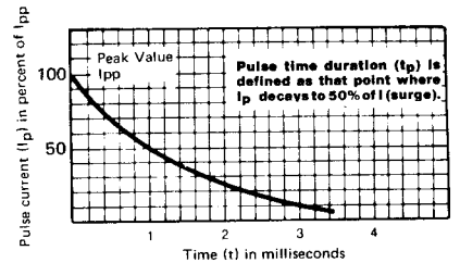
FIG. 2. Pulse wave form for exponential surge
