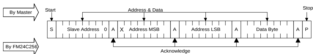
Figure 5. Single Byte Write
