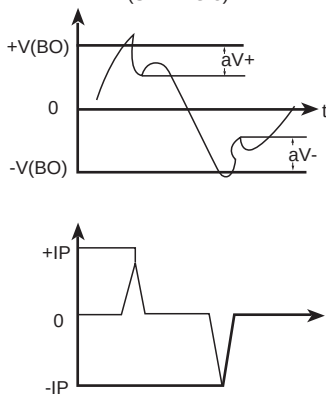
FIG.4-TEST CIRCUIT WAVE FORMS (SEE FIG.5)
