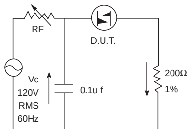
FIG.5-CIRCUIT USED TO MEASURE DIAC CHARACTERISTICS
