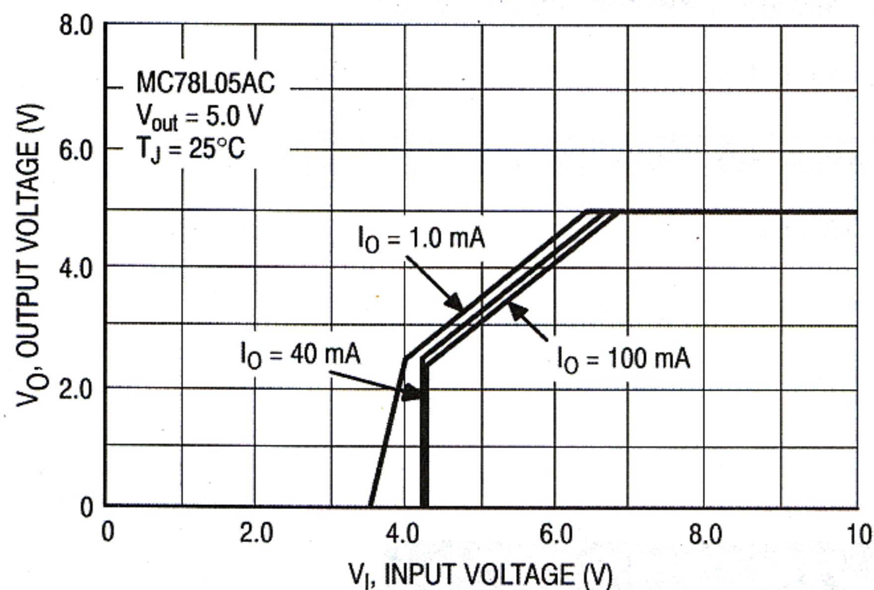
Dropout Characteristics
