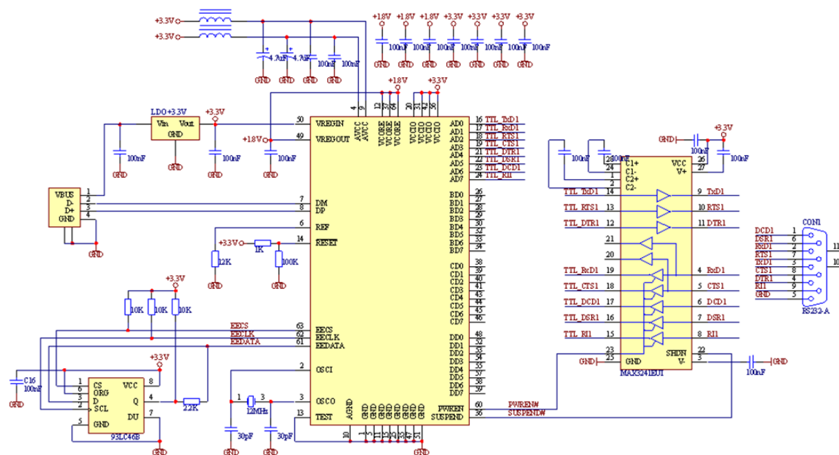
Figure 4.1 RS232 Configuration
