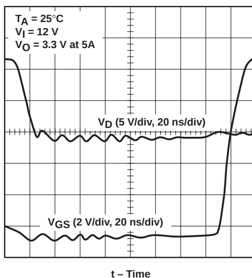
Figure 52. Q1 Drain Voltage vs Q2 Gate-Source Voltage
