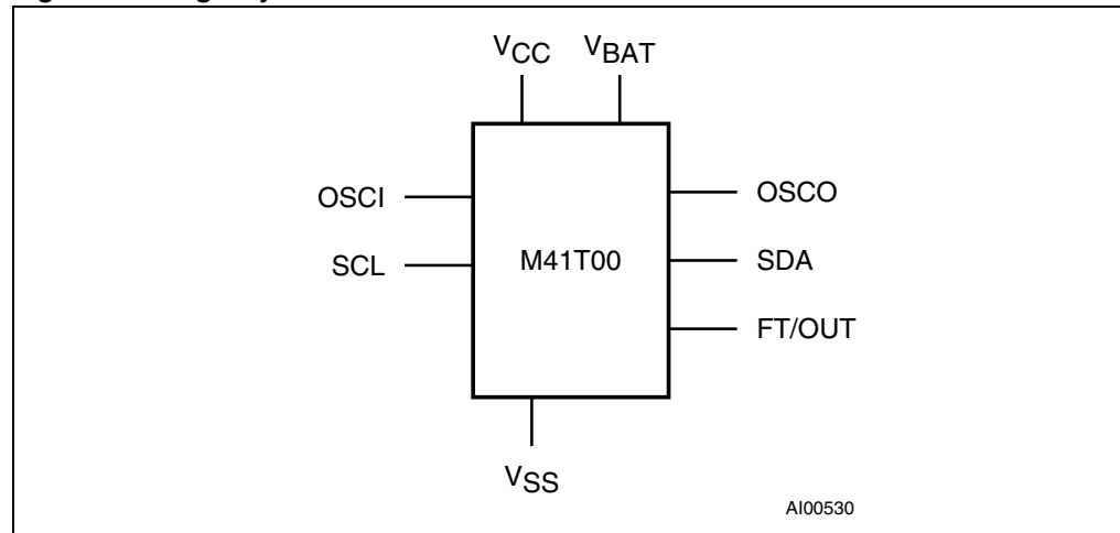
Figure 1. Logic symbol
