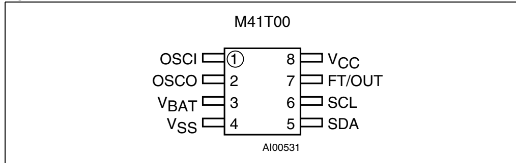
Figure 2. SOIC connection
