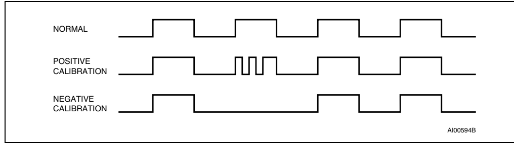
Figure 13. Clock calibration
