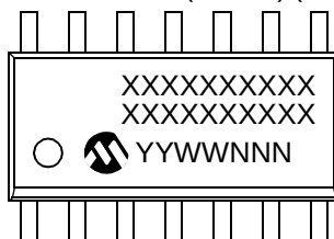
14-Lead SOIC (150 mil) (MCP6144)
