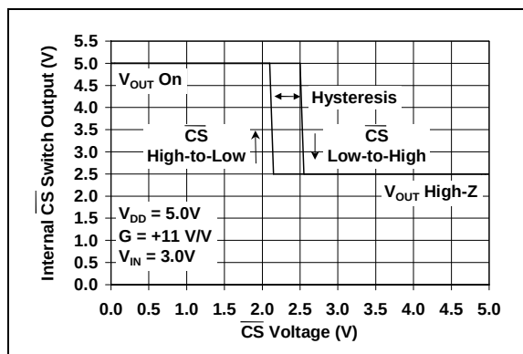
FIGURE 2-34: Internal Chip Select ( \overline{\text{CS}} ) Hysteresis (MCP6143 only).
