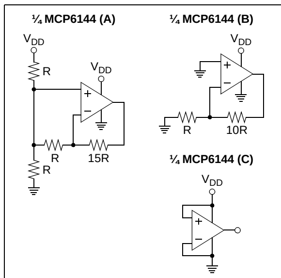
FIGURE 4-7: Unused Op Amps.
