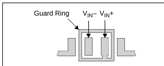
FIGURE 4-8: Example Guard Ring Layout for Inverting Gain.
