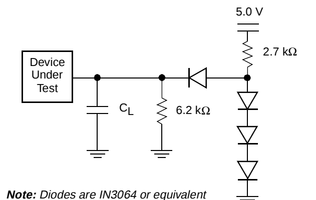
Figure 8. Test Setup
