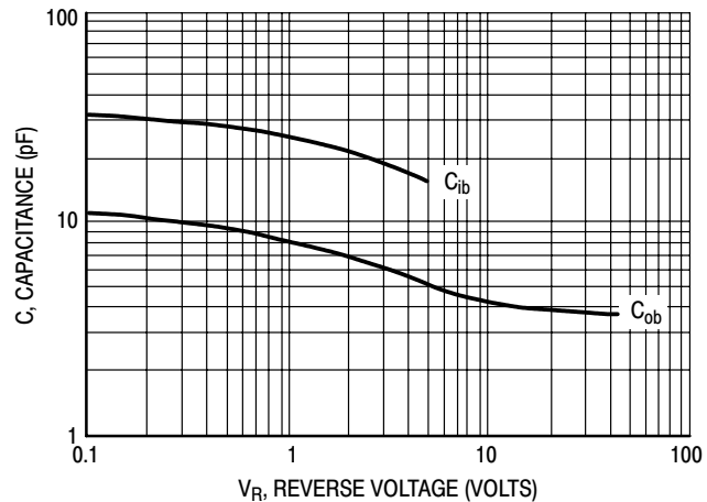
Figure 5. Capacitances
