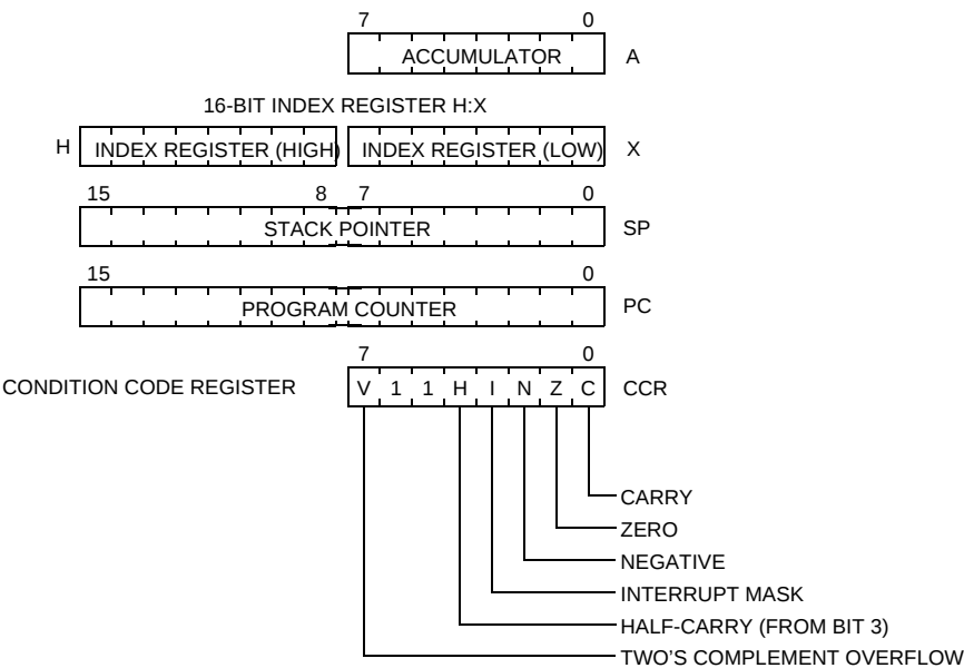
Figure 18. CPU Registers
