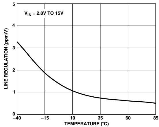
TPC 10. ADR381 Line Regulation vs. Temperature
