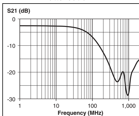
Figure 4. USBUFxxW6 typical attenuation
