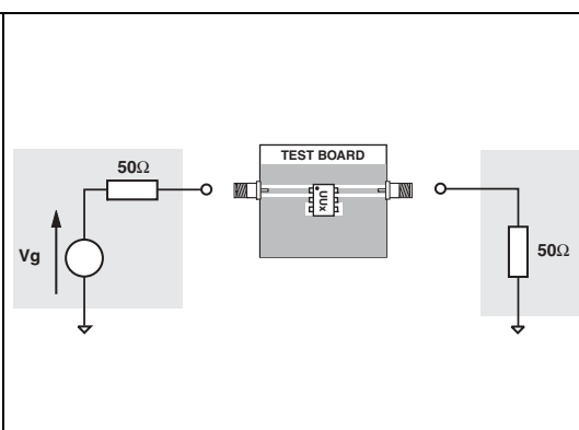
Figure 5. Measurement configuration
