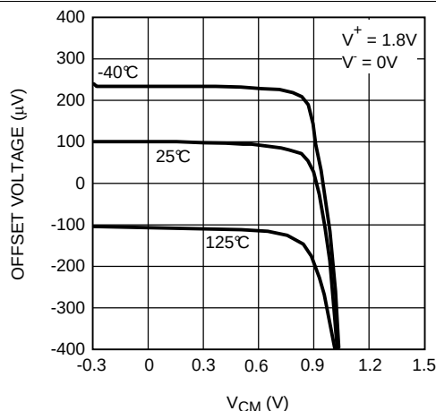
Figure 10. Offset Voltage vs. V_{CM}
