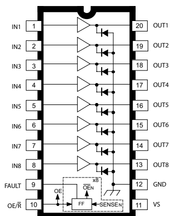
Pin-Out Diagram
