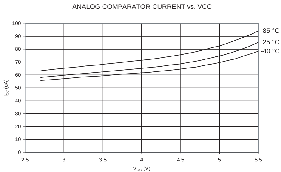
Figure 208. Analog Comparator Current vs. V_{CC}
