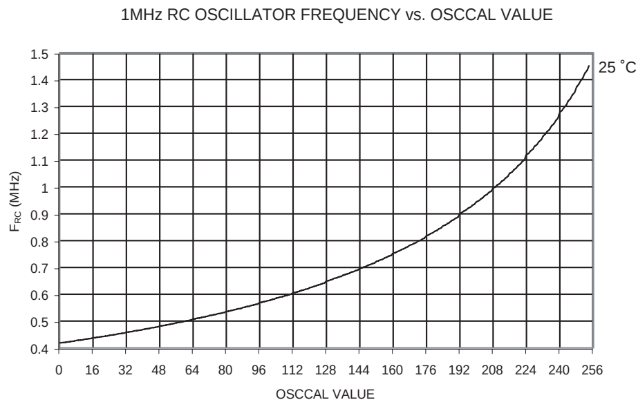
Figure 195. 1 MHz RC Oscillator Frequency vs. Oscscal Value
