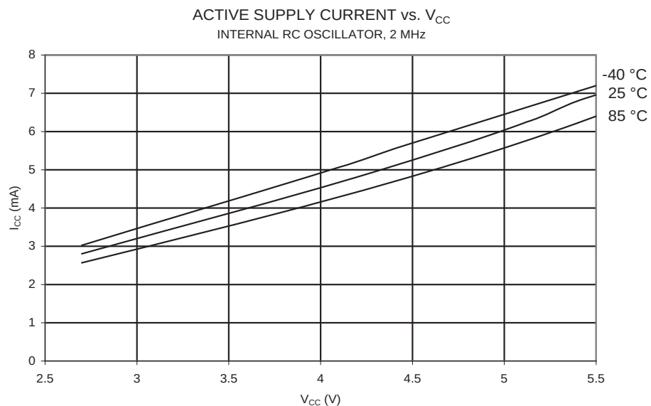
Figure 164. Active Supply Current vs. V_{CC} (Internal RC Oscillator, 2 MHz)
