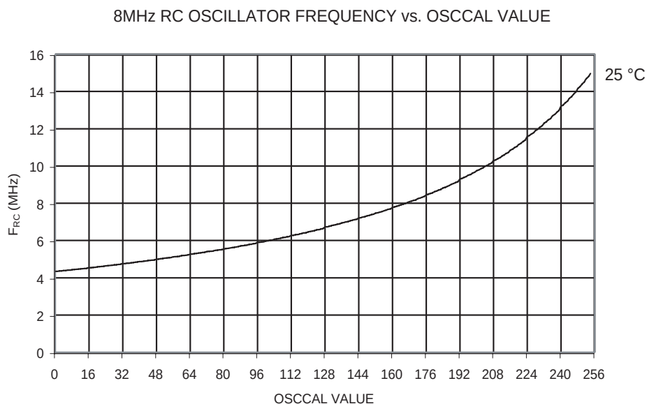
Figure 204. 8 MHz RC Oscillator Frequency vs. Oscscal Value
