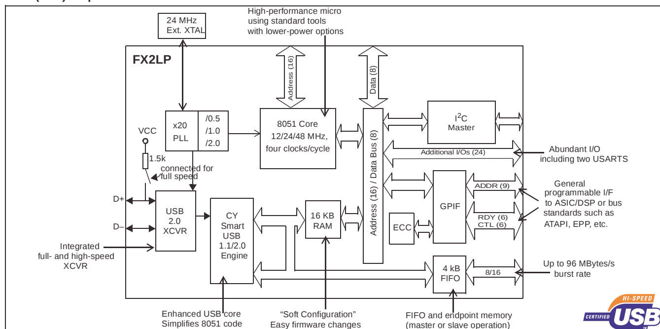
Figure 1-1. Block Diagram
