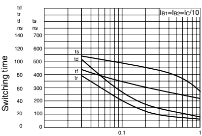
Switching Speeds
