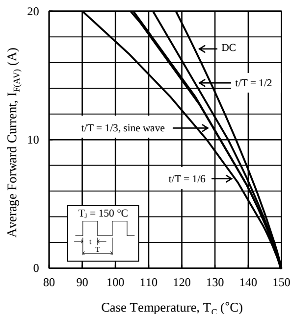
Figure 2. I_{F(AV)} vs. T_C Typical Characteristics ( V_R = 200\text{ V} )
