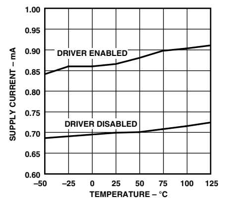
Figure 19. Supply Current vs. Temperature
